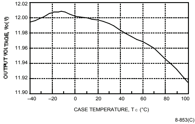
Figure 6. CC030B Typical Output Voltage Variation over Ambient Temperature Range
