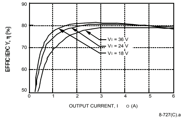
Figure 8. CC030A Typical Converter Efficiency vs. Output Current
