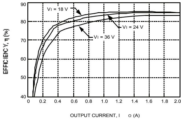
Figure 10. CC030C Typical Converter Efficiency vs. Output Current
