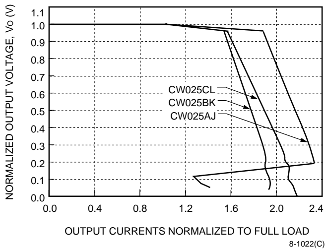
Figure 2. CW025 Dual Output-Series Normalized Output Current vs. Normalized Output Voltage at V_i = 48\text{ V} and T_c = 25\text{ }^\circ\text{C}
