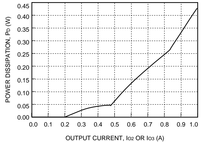
Figure 26. CW025ABK-M, Losses Associated with ±12 V Output, Ps2/Ps3
