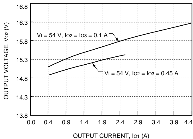
Figure 8. CW025ACL-M Typical Cross Regulation with Respect to I_{o1}
