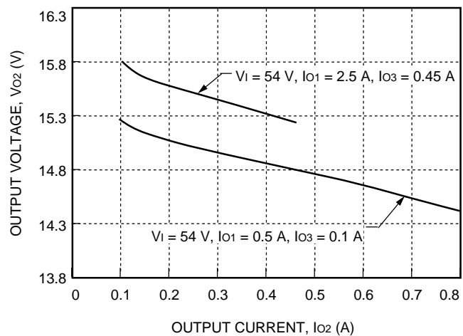
Figure 7. CW025ACL-M Typical Load Regulation
