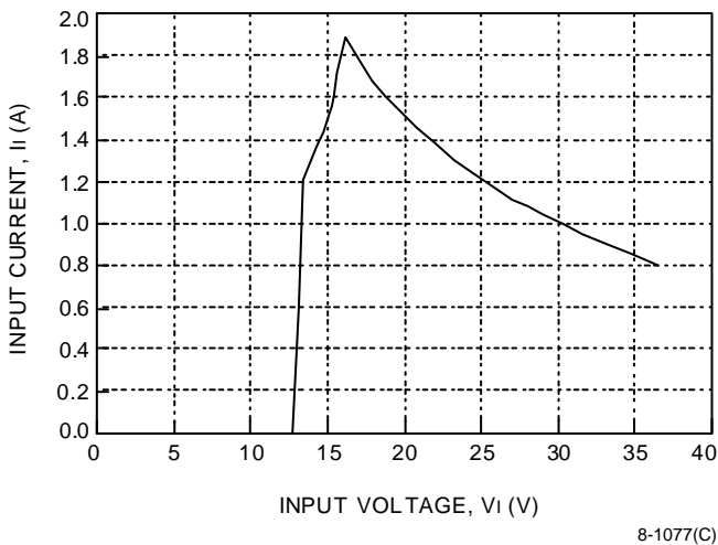
Figure 1. DC025 Triple Output-Series Typical Input Characteristics
