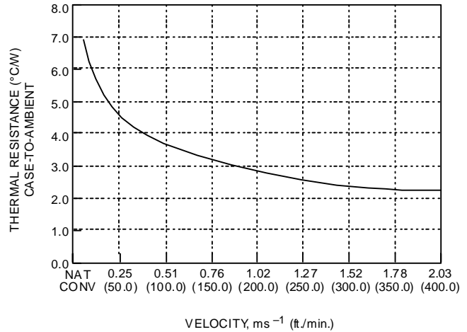
Figure 29. Case-to-Ambient Thermal Resistance vs. Air Velocity
