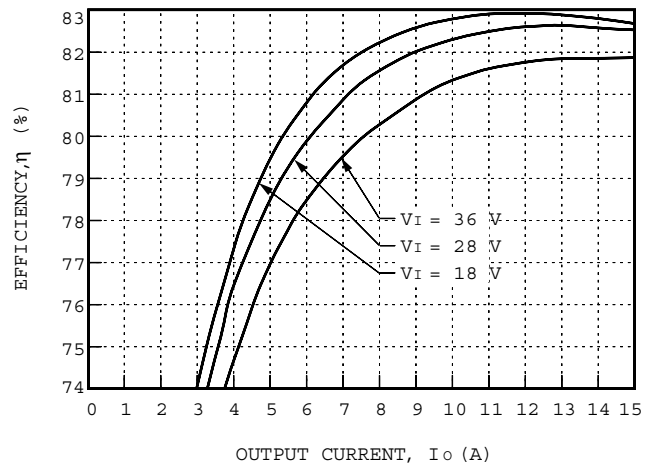
Figure 8. Typical JC075A Converter Efficiency vs. Output Current at Room Temperature
