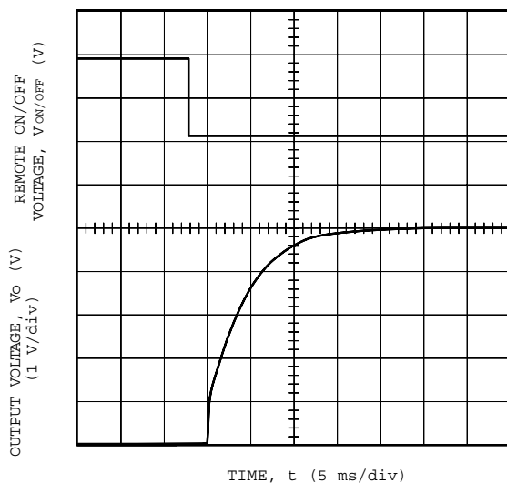
Figure 13. Typical Start-Up from Remote On/Off JC100A1; I_o = \text{Full Load}
