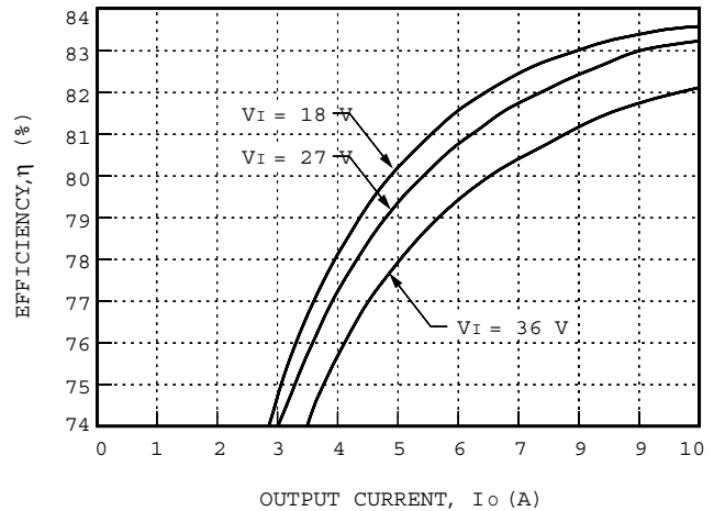
Figure 7. Typical JC050A Converter Efficiency vs. Output Current at Room Temperature
