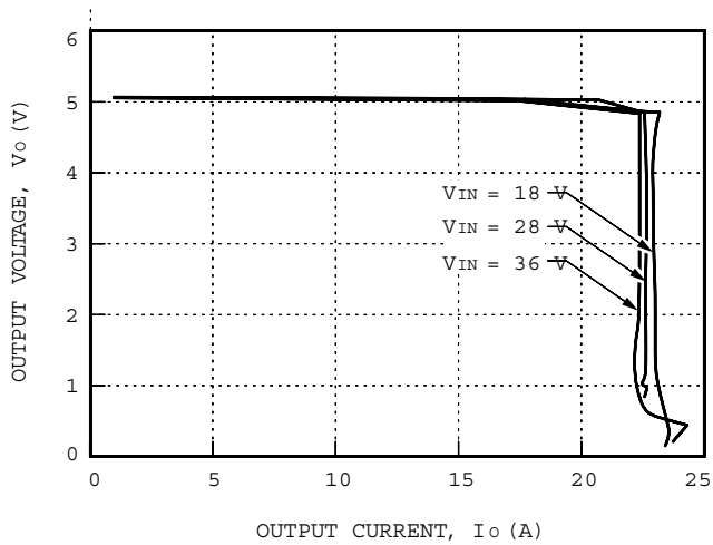
Figure 6. Typical JC100A Output Characteristics at Room Temperature.
