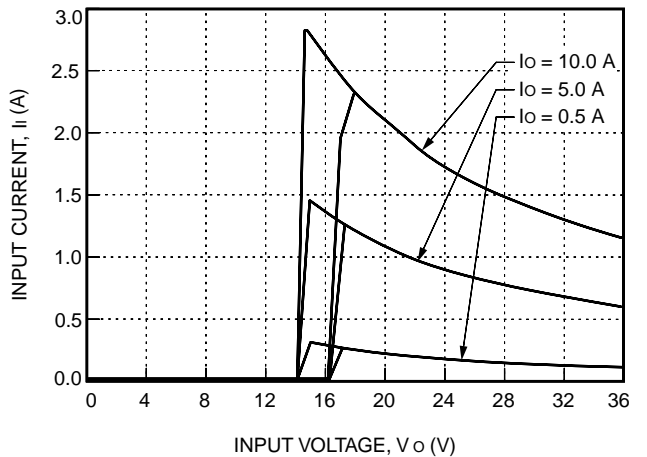
Figure 1. Typical JC050F Input Characteristics at Room Temperature
