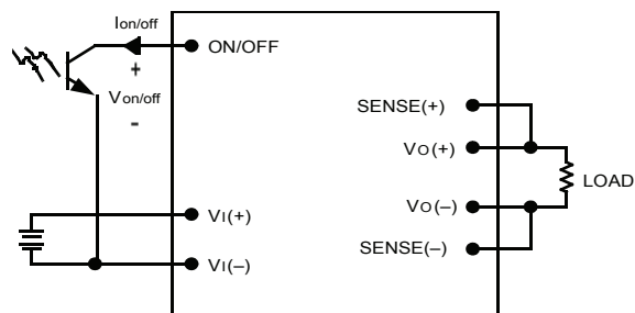
Figure 23. Remote On/Off Implementation
