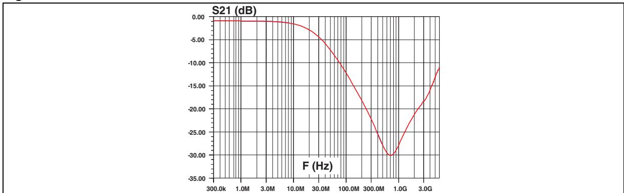
Figure 5. ESD response to IEC 61000-4-2 +15 kV air discharge on SPK R line
