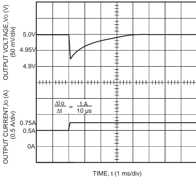
Figure 25. ME005A Typical Output Voltage Waveform for a Step Load Change from 50% to 75% of I_{o,max} with V_i = 48\text{ V} and T_A = 25\text{ }^\circ\text{C} (ME005N Waveform Is Similar, but with 5.2 V Steady-State.)
