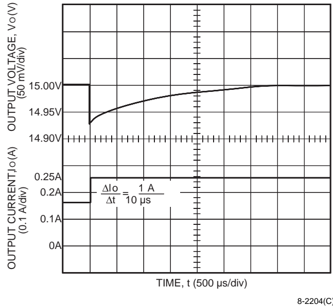
Figure 27. ME005C Typical Output Voltage Waveform for a Step Load Change from 50% to 75% of I_{o,max} with V_i = 48\text{ V} and T_A = 25\text{ }^\circ\text{C}
