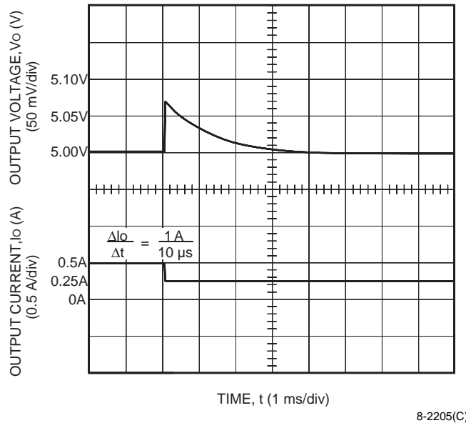
Figure 28. ME005A Typical Output Voltage Waveform for a Step Load Change from 50% to 25% of I_{o,max} with V_i = 48\text{ V} and T_A = 25\text{ }^\circ\text{C} (ME005N Waveform Is Similar, but with 5.2 V Steady-State.)
