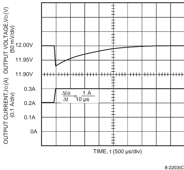
Figure 26. ME005B Typical Output Voltage Waveform for a Step Load Change from 50% to 75% of I_{o,max} with V_i = 48\text{ V} and T_A = 25\text{ }^\circ\text{C}
