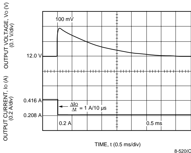
Figure 14. MW010B Typical Output Voltage Waveform for a Step Load Change from 50% to 25% of I_{o,max} ; V_i = 48\text{ V} ; T_A = 25\text{ }^\circ\text{C}
