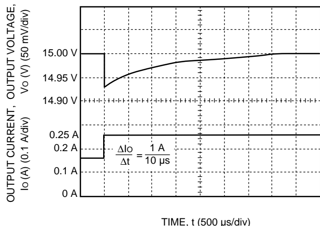
Figure 23. MW005C Typical Output Voltage Waveform for a Step Load Change from 50% to 75% of I_{o,max} with V_i = 48\text{ V} and T_A = 25\text{ }^\circ\text{C}
