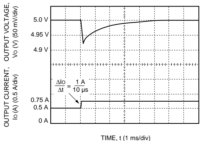
Figure 21. MW005A Typical Output Voltage Waveform for a Step Load Change from 50% to 75% of I_{o,max} with V_i = 48\text{ V} and T_A = 25\text{ }^\circ\text{C}
