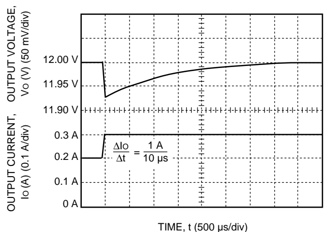
Figure 22. MW005B Typical Output Voltage Waveform for a Step Load Change from 50% to 75% of I_{o,max} with V_i = 48\text{ V} and T_A = 25\text{ }^\circ\text{C}
