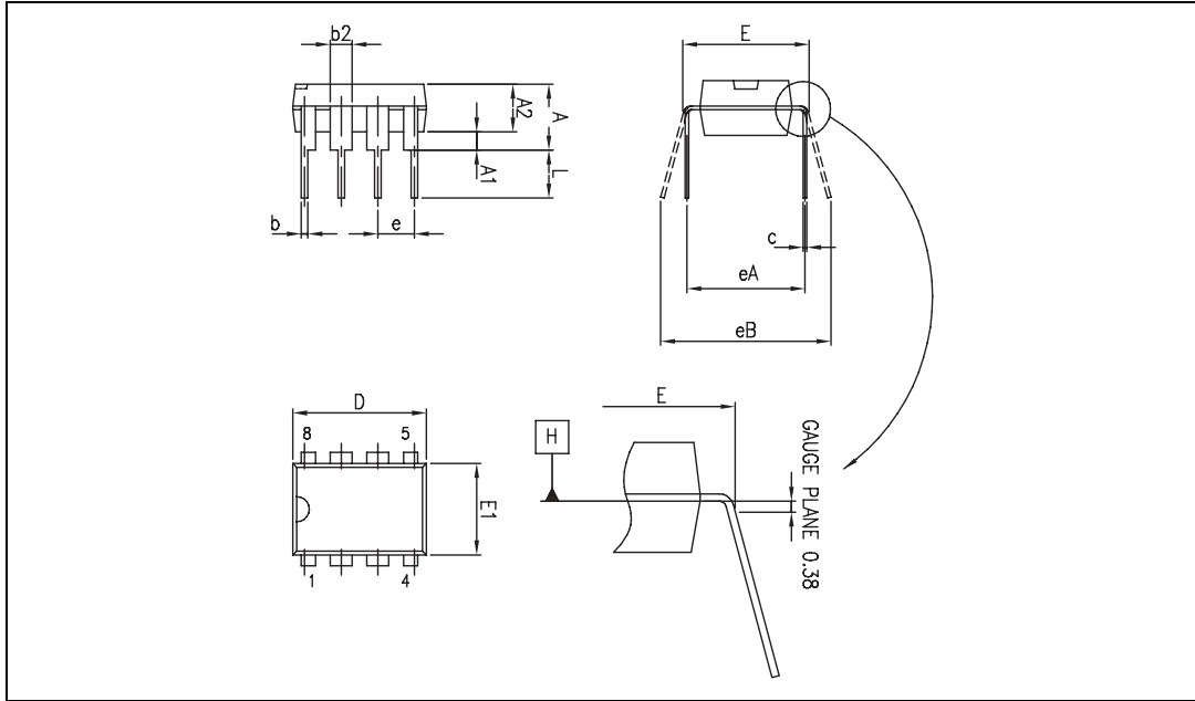
Figure 15. DIP8 package mechanical drawing
