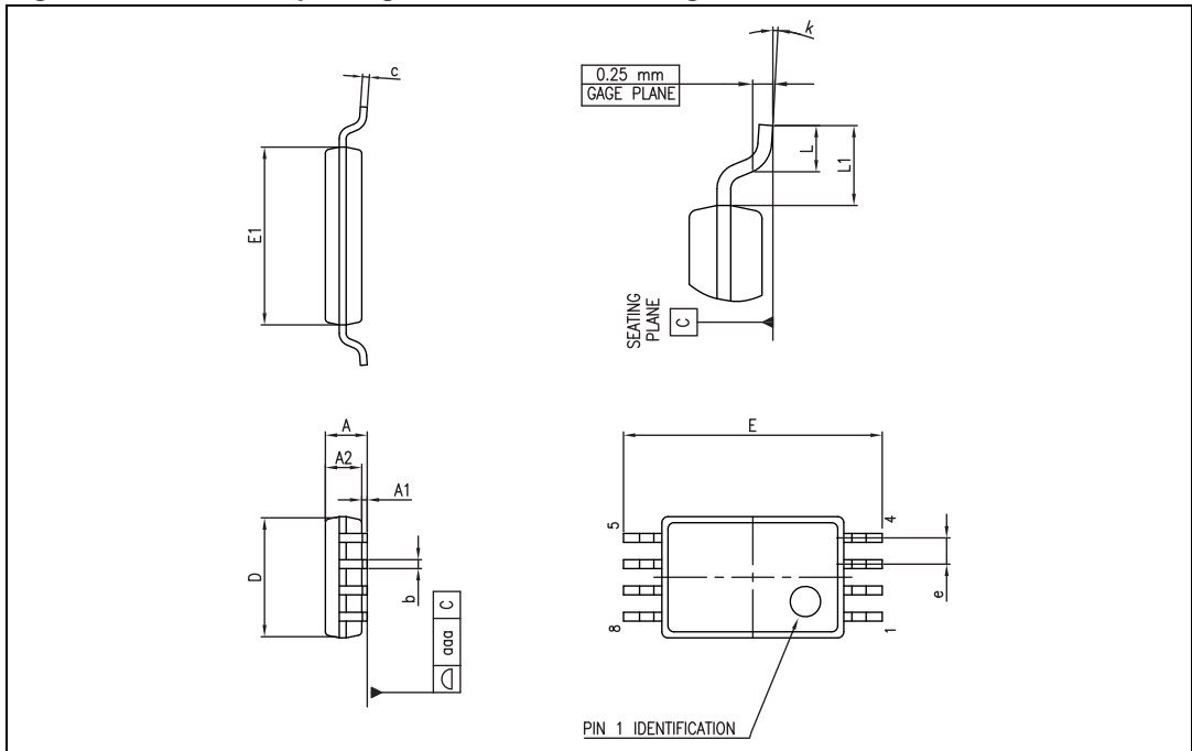
Figure 50. TSSOP8 package mechanical drawing
