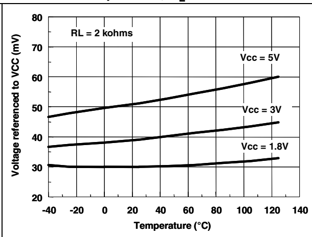
Figure 18. Low level output voltage vs. temperature, RL = 2 kΩ
