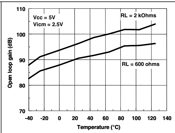
Figure 14. Open loop gain vs. temperature at Vcc = 5 V
