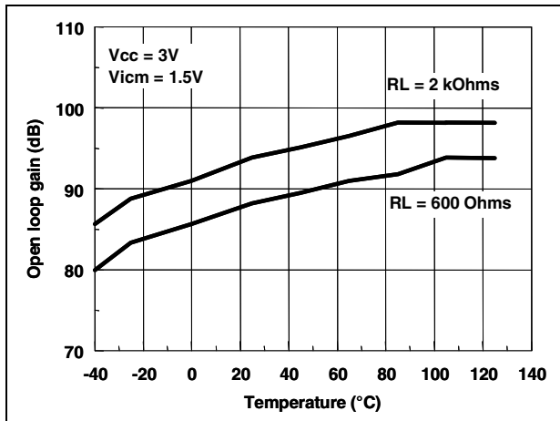
Figure 13. Open loop gain vs. temperature at Vcc = 3 V
