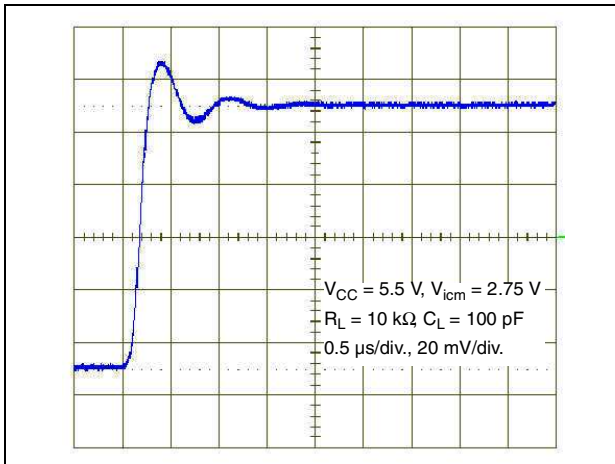
Figure 21. Response to a 100 mV input step for gain = 1 at V_{CC} = 5.5 V rising edge
