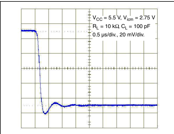
Figure 22. Response to a 100 mV input step for gain = 1 at V_{CC} = 5.5 V falling edge
