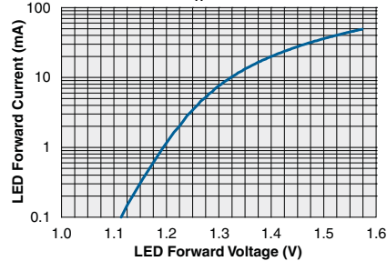
LED Voltage vs. Current (Log) ( T_A=25^\circ\text{C} )
