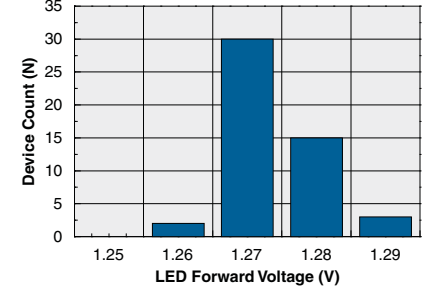
Typical LED Forward Voltage Drop (N=50, I_F=5\text{mA} , T_A=25^\circ\text{C} )
