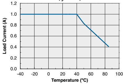
Form-A Relay Typical Load Current vs. Temperature ( I_F=5mA )
