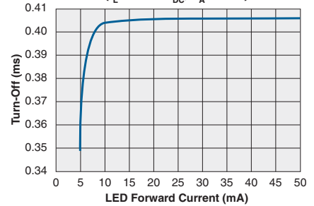
Typical Turn-Off vs. LED Forward Current ( I_L=170\text{mA}_{DC} , T_A=25^\circ\text{C} )
