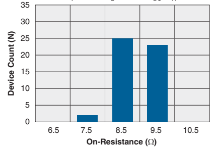
Typical On-Resistance Distribution (N=50, I_F=5\text{mA} , I_L=170\text{mA}_{DC} , T_A=25^\circ\text{C} )
