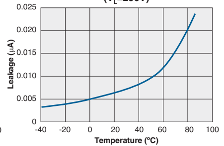
Typical Leakage vs. Temperature Measured across Pins 5&6 or 7&8 ( V_L=250V )
