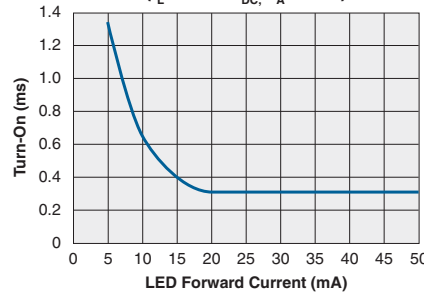
Typical Turn-On vs. LED Forward Current ( I_L=170\text{mA}_{DC} , T_A=25^\circ\text{C} )
