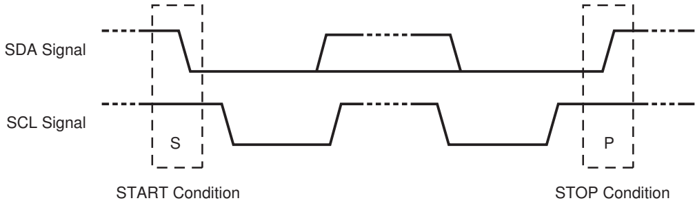
Figure 31. START and STOP Conditions In I 2 C Protocol
