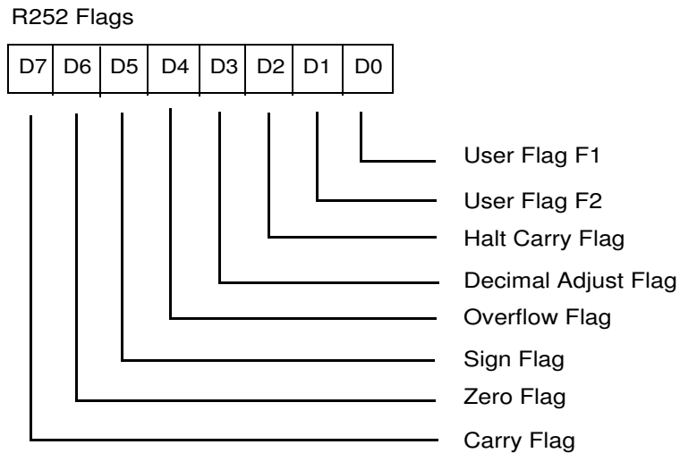
Figure 52. Flag Register (FC n : Read/Write)
