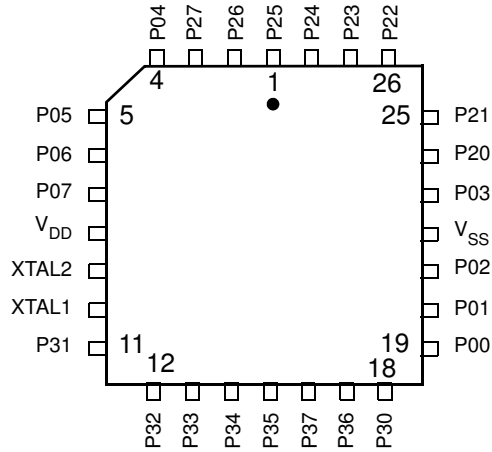
Figure 10. Standard Mode 28-Pin PLCC Pin Configuration
