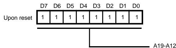
Figure 56. RAMLBR (Z180 MPU Read/Write, Address xxE7H)
