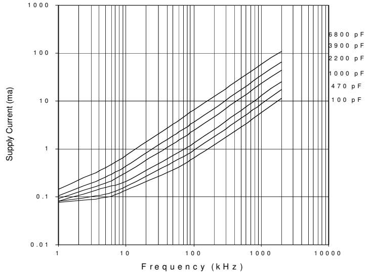
Fig. 14 Supply Current vs. Frequency Vcc = 12V
