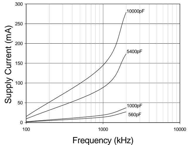
Fig. 21 Supply Current vs. Frequency V_{SUPPLY} = 15V
