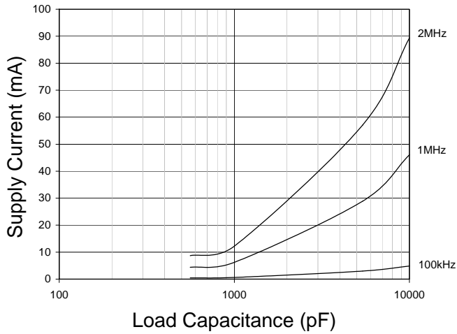
Fig. 16 Supply Current vs. Capacitive Load V_{SUPPLY} = 5V
