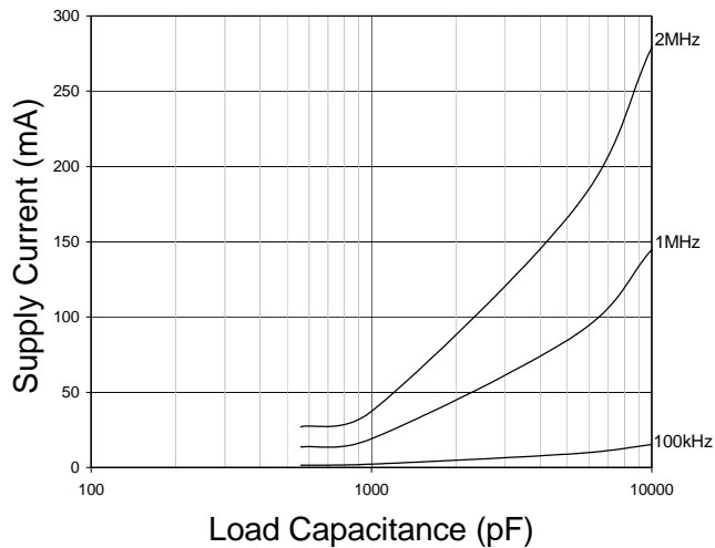
Fig. 20 Supply Current vs. Capacitive Load V_{SUPPLY} = 15V
