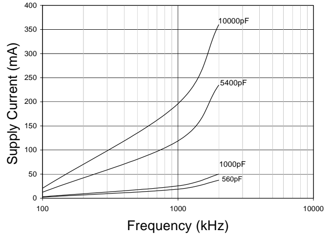
Supply Current vs. Frequency V_{\text{SUPPLY}} = 20\text{V}
