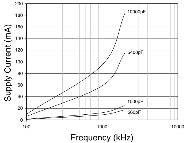
Fig. 19 Supply Current vs. Frequency V_{SUPPLY} = 10V
