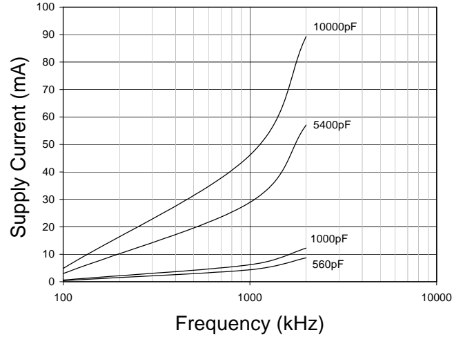
Fig. 17 Supply Current vs. Frequency V_{SUPPLY} = 5V
