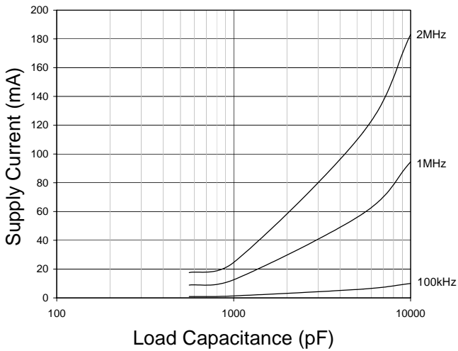
Fig. 18 Supply Current vs. Capacitive Load V_{SUPPLY} = 10V
