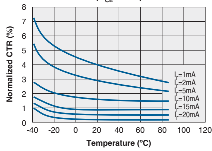
Typical Normalized CTR vs. Temperature ( V_{CE}=0.5V )
