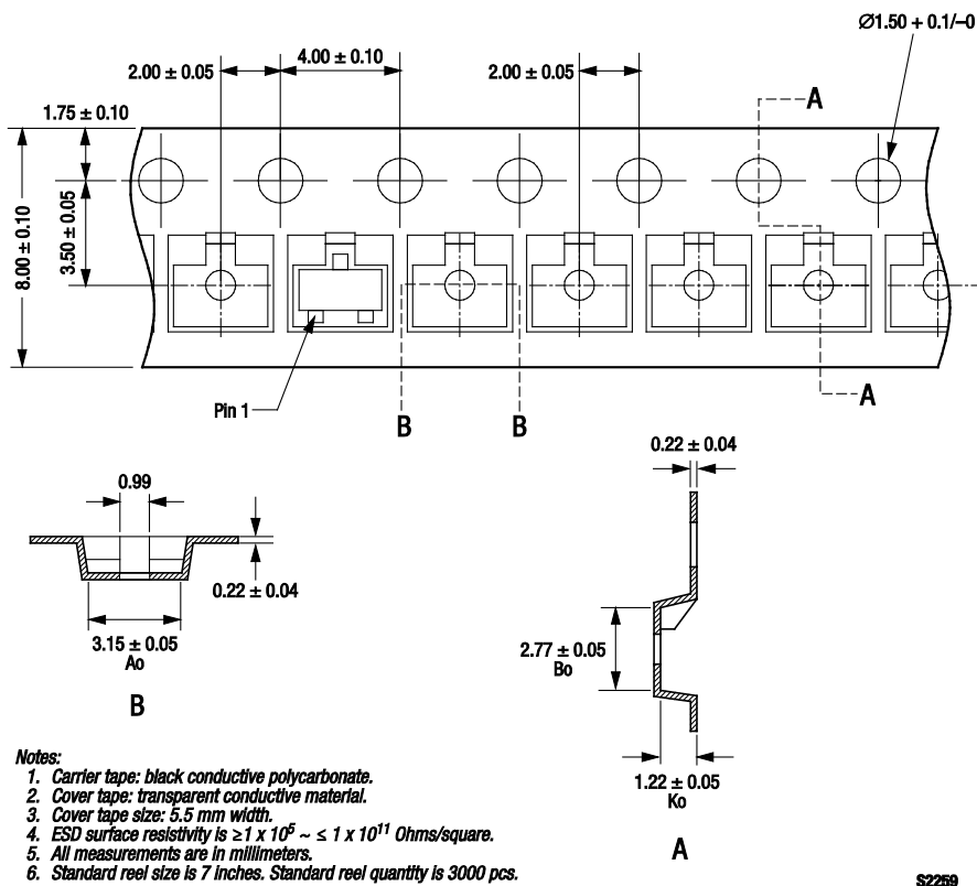
Figure 10. SOT-23 Tape and Reel Dimensions
