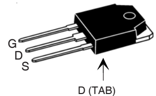
TO-247 (IXTH)
