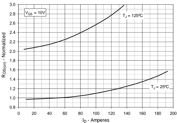
Fig. 5. R_{DS(on)} Normalized to I_D = 49A Value vs. Drain Current
