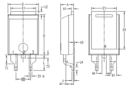
PLUS220SMD (IXFV_S) Outline
