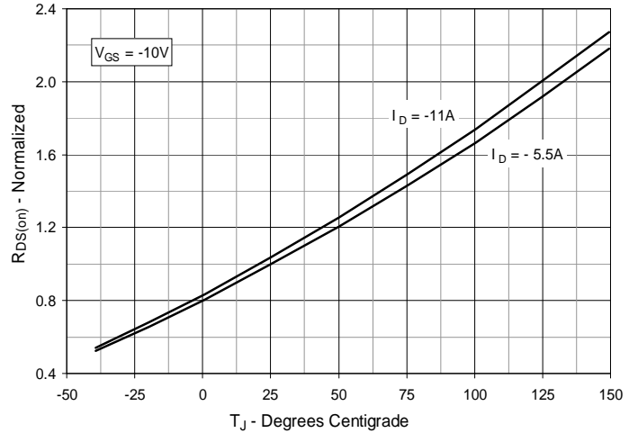
Fig. 4. R_{DS(on)} Normalized to I_D = -5.5\text{A} vs. Junction Temperature
