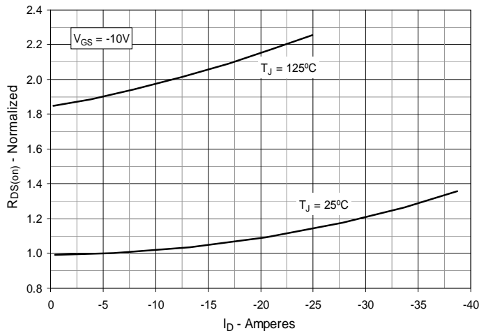
Fig. 5. R_{DS(on)} Normalized to I_D = -5.5\text{A} vs. Drain Current
