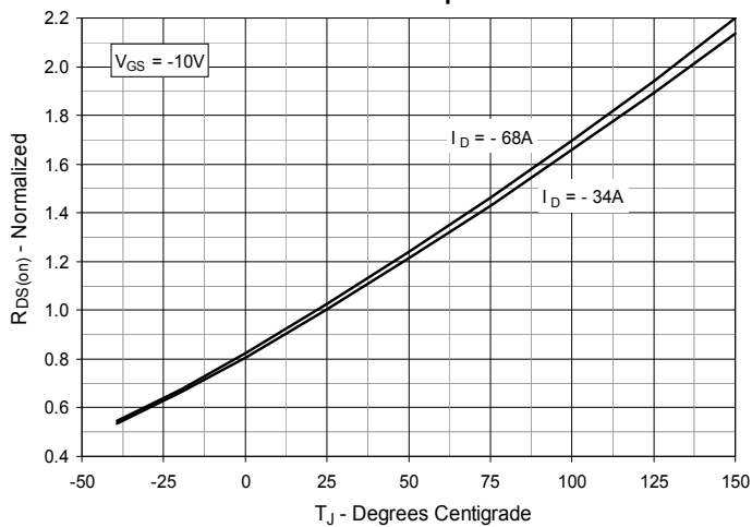
Fig. 4. R_{DS(on)} Normalized to I_D = -34\text{A} vs. Junction Temperature
