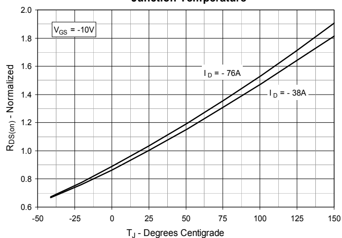
Fig. 4. R_{DS(on)} Normalized to I_D = -38\text{A} vs. Junction Temperature
