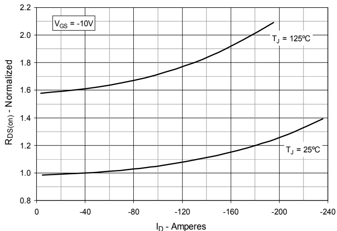
Fig. 5. R_{DS(on)} Normalized to I_D = -38\text{A} vs. Drain Current
