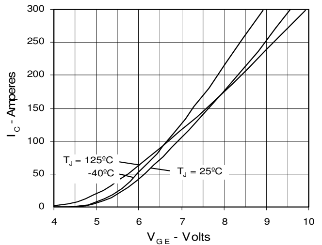
Fig. 6. Input Admittance
