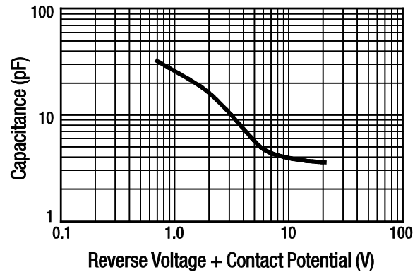
Figure 2. Capacitance vs Reverse Voltage + Contact Potential
