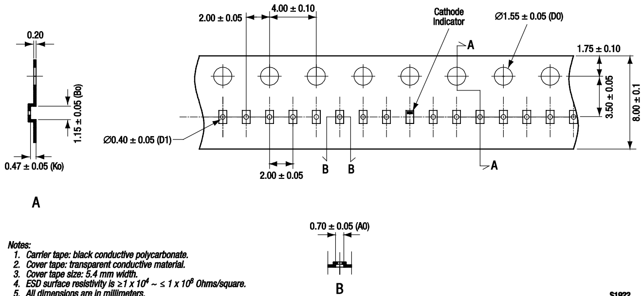
Figure 7. SMV1705-040LF Tape and Reel Dimensions
