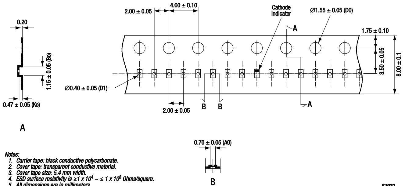
Figure 7. SMV1232-040LF Tape and Reel Dimensions
