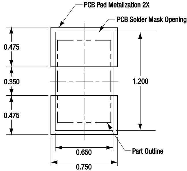
Figure 4. SMV1232-040LF PCB Layout Footprint
