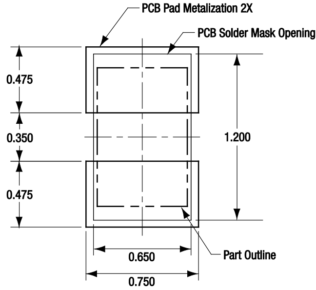
Figure 4. SMV2019-040LF PCB Layout Footprint
