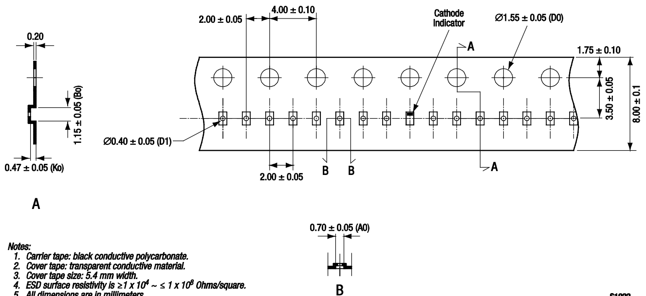
Figure 7. SMV2019-040LF Tape and Reel Dimensions
