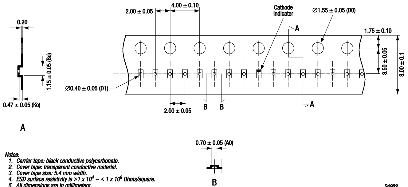
Figure 7. SMV1231-040LF Tape and Reel Dimensions
