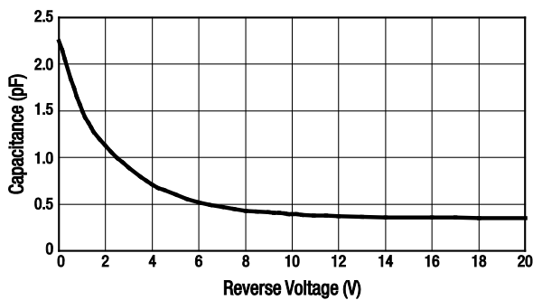
Figure 1. Capacitance vs Reverse Voltage
