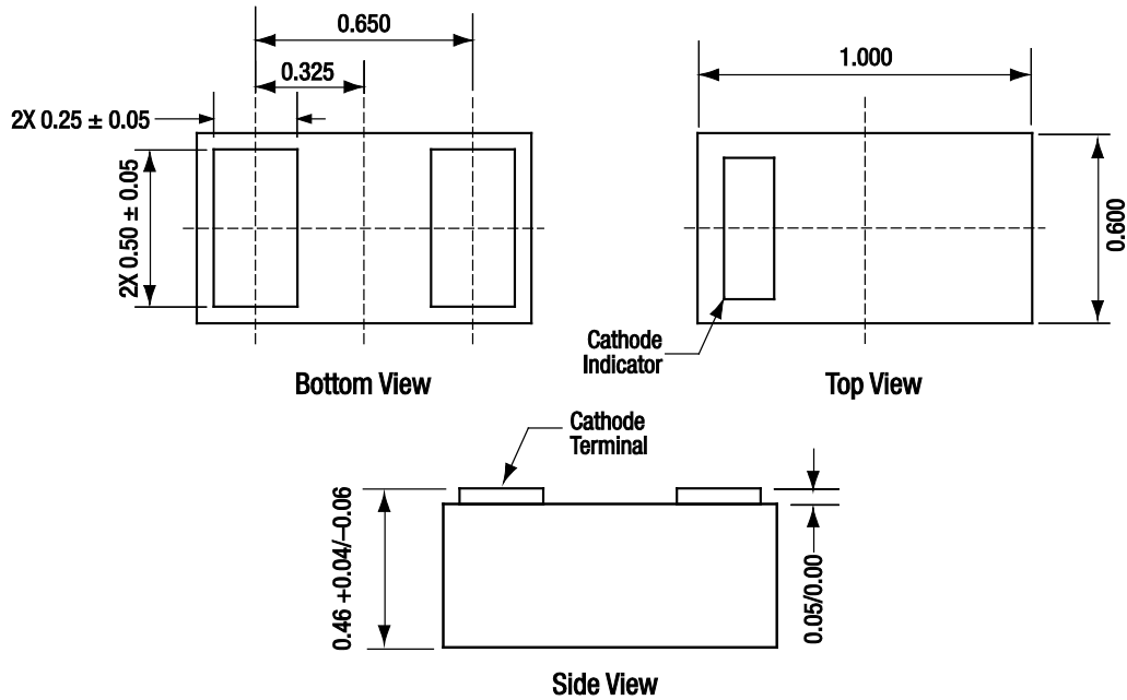
Figure 6. SMV1231-040LF Package Dimensions
