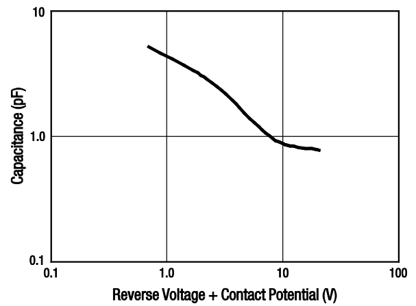
Figure 2. Capacitance vs Reverse Voltage + Contact Potential
