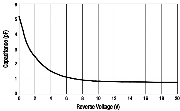
Figure 1. Capacitance vs Reverse Voltage
