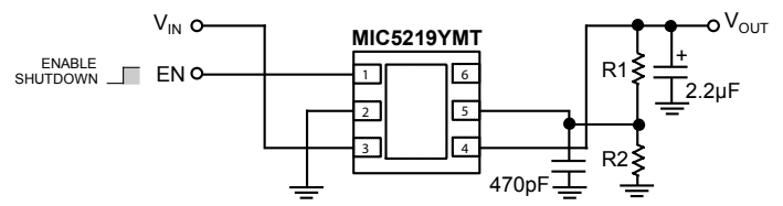
Ultra-Low-Noise Regulator (Adjustable)
