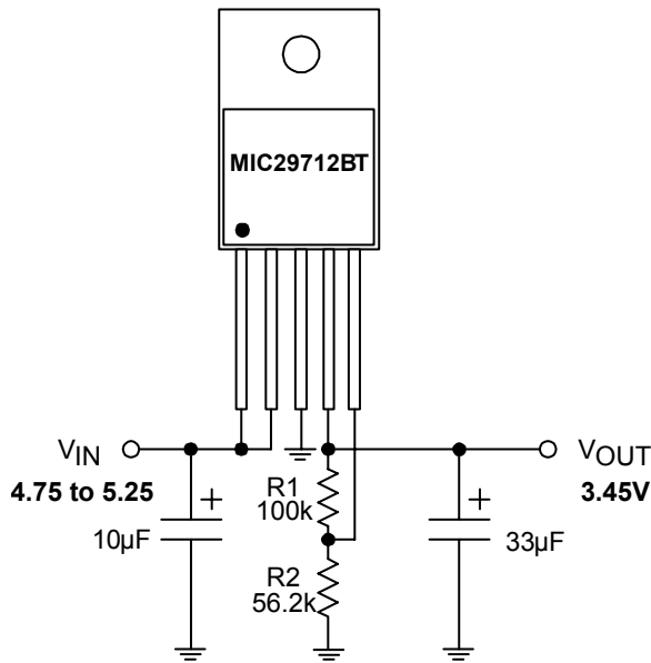
Figure 4. Adjustable Regulator with Resistors
