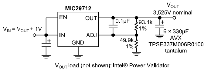
MIC29710 Load Transient Response Test Circuit
