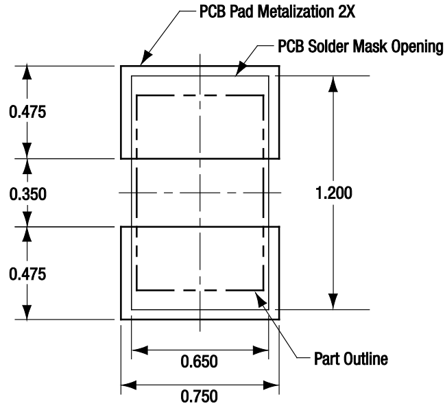
Figure 4. SMV1236-040LF PCB Layout Footprint
