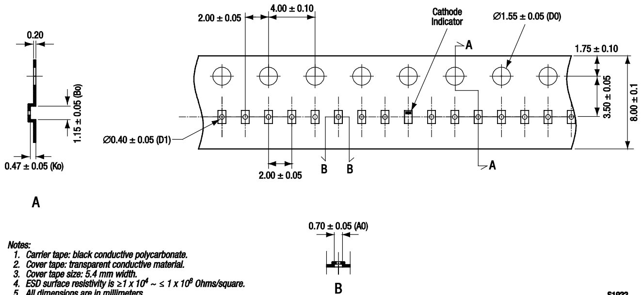
Figure 7. SMV1236-040LF Tape and Reel Dimensions
