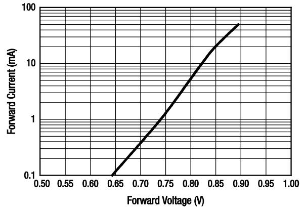
Figure 2. DC Characteristic
