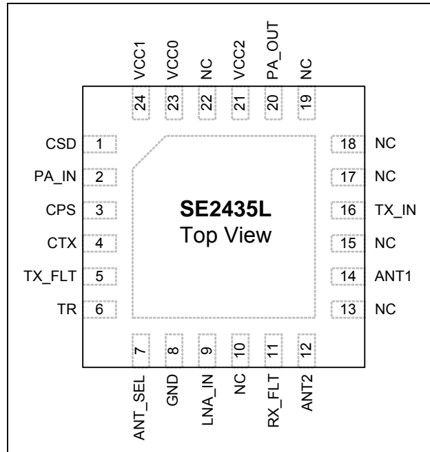
Figure 2: SE2435L Pinout
