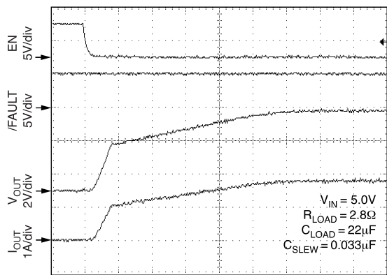
Output Slew Response
