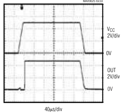
POWER-UP/POWER-DOWN RESPONSE
