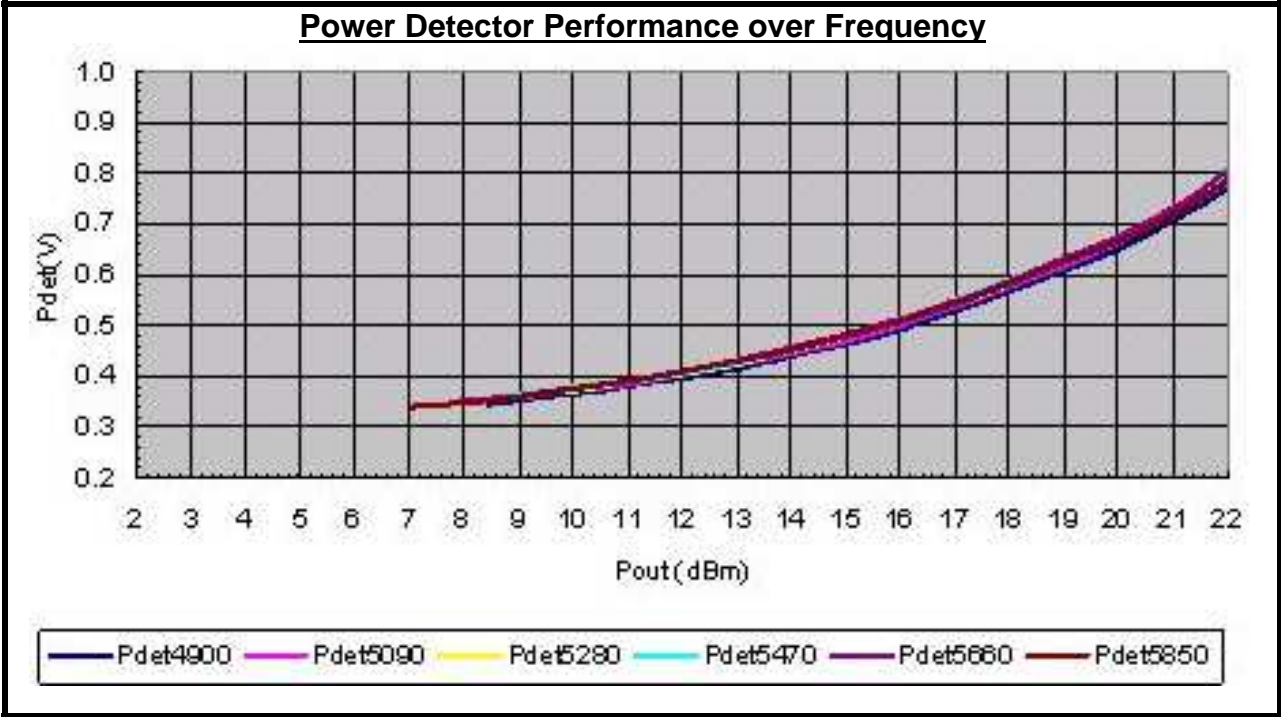
Figure 3: SE5007BT Power Detector Characteristic
