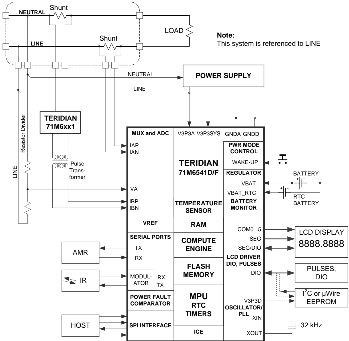
Figure 36: 71M6541D/F/G with 71M6x01 isolated Sensor
