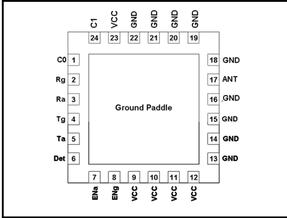
Figure 2: SE5512L Pin Out (Top View Through Package)
