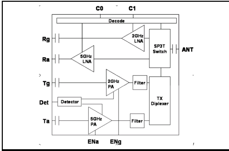
Figure 1: SE5512L Functional Block Diagram
