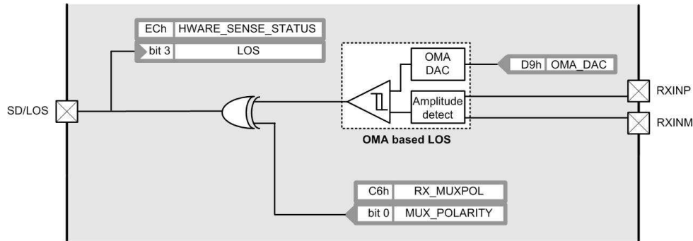
Figure 15 - LOS Detection
