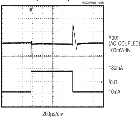
LOAD-TRANSIENT RESPONSE (5V OUTPUT)
