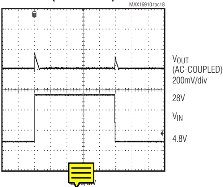
LINE-TRANSIENT RESPONSE (3.3V OUTPUT)
