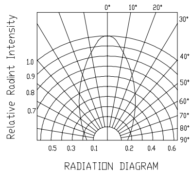
Radiation Diagram Ta=25°
